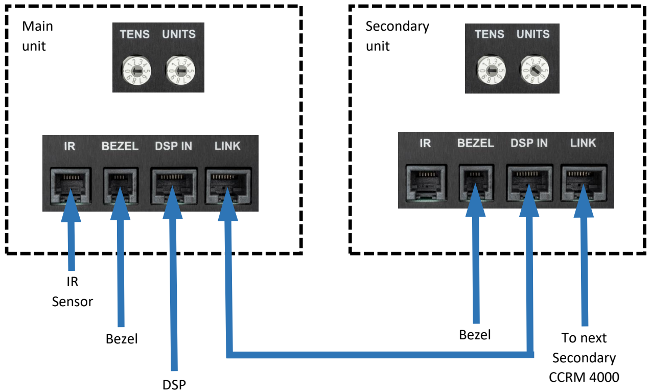
Main / Secondary CCRM 4000 Connectivity Diagram
